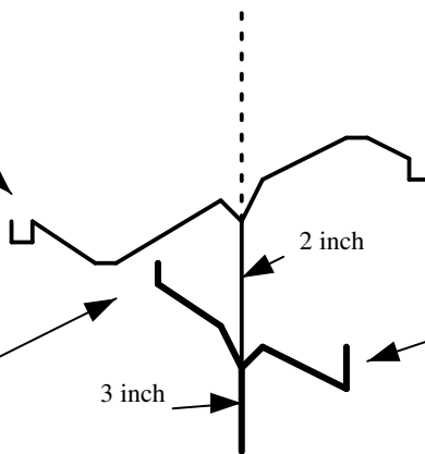
Common vents serving as a wet vent
