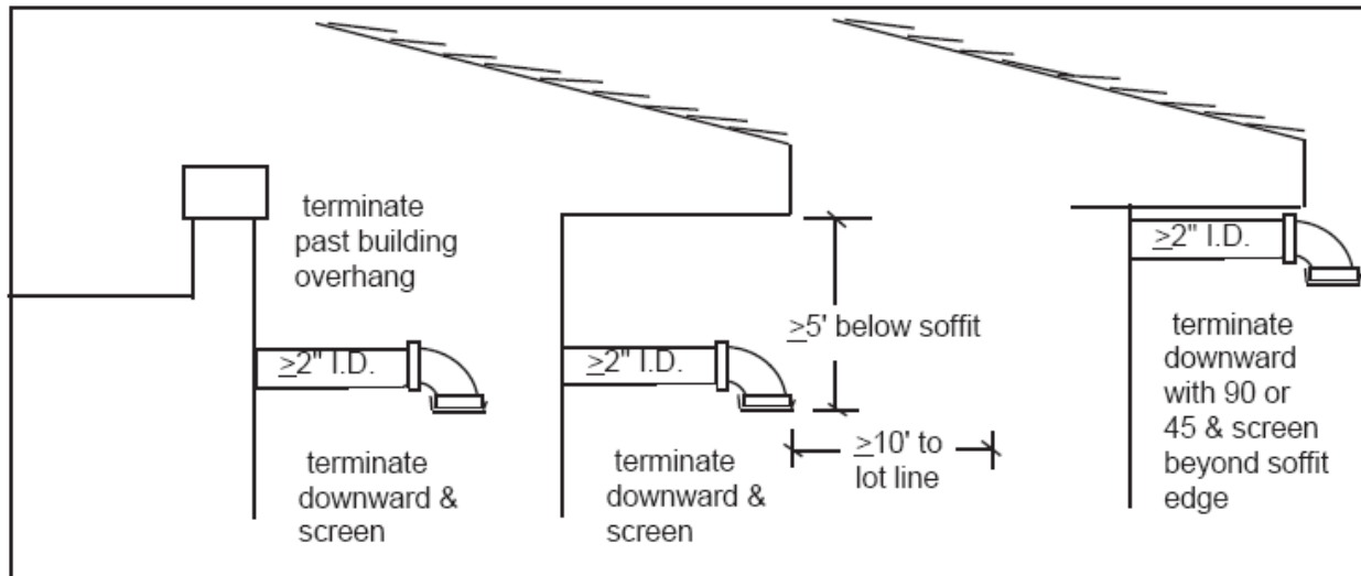
VENTS TERMINATING THROUGH WALLS
