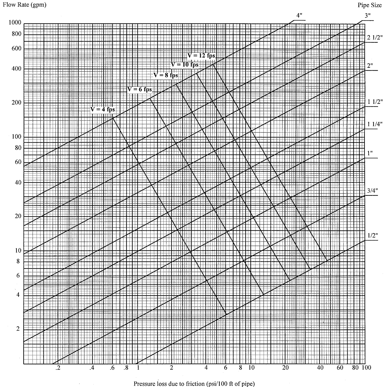
Graph A-382.40 (7)-2 PRESSURE LOSSES DUE TO FLOW FRICTION Material: Copper Tube-Type K, ASTM B88; (C = 150)
