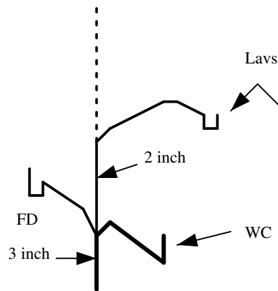
Individual vent serving as a wet vent
