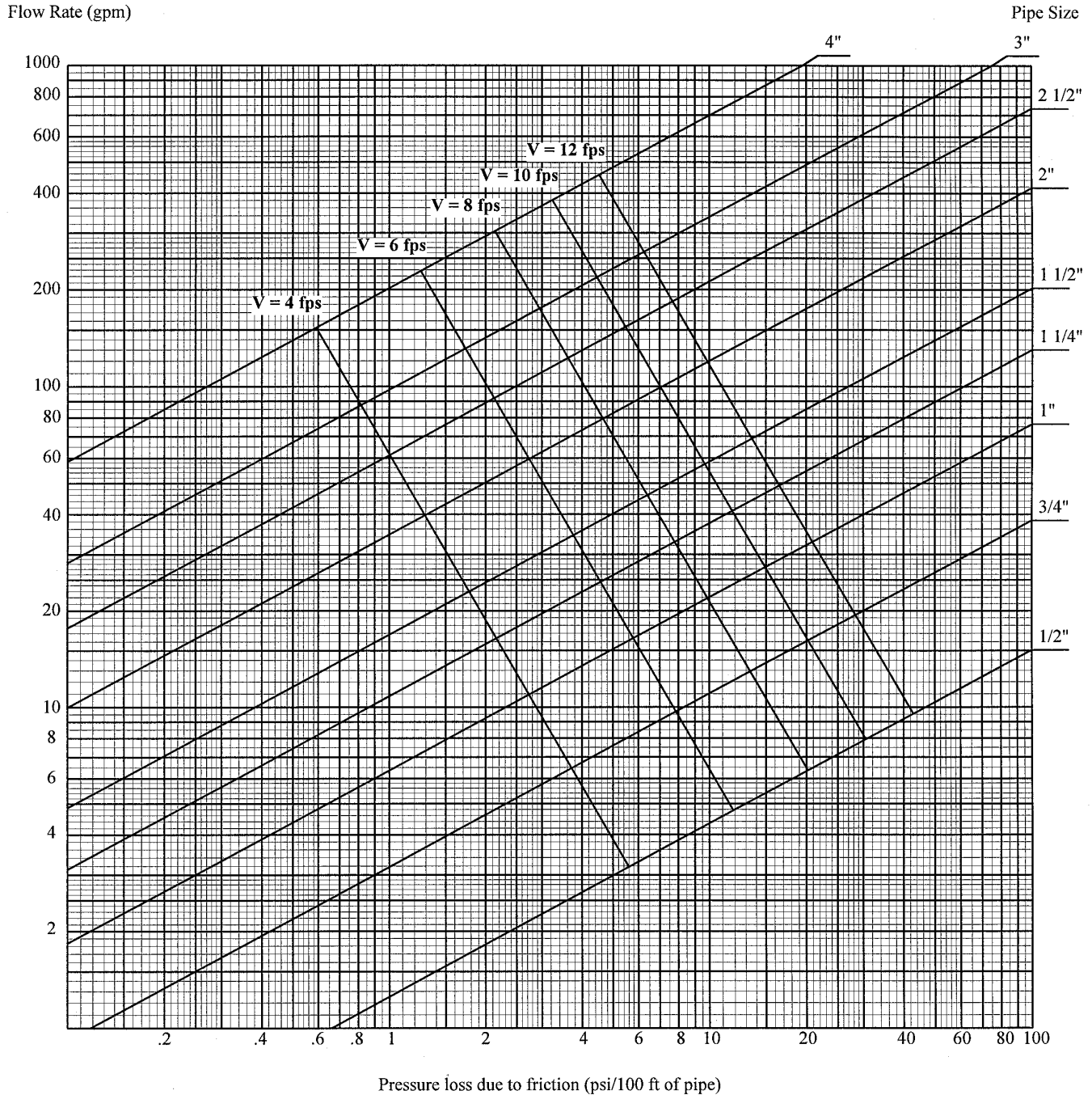
Graph A-382.40 (7)-9 PRESSURE LOSSES DUE TO FLOW FRICTION Material: Copper Tube-Type M, ASTM B88; (C = 150)
