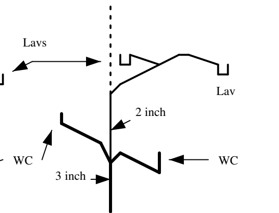
Common vents serving as a wet vent
